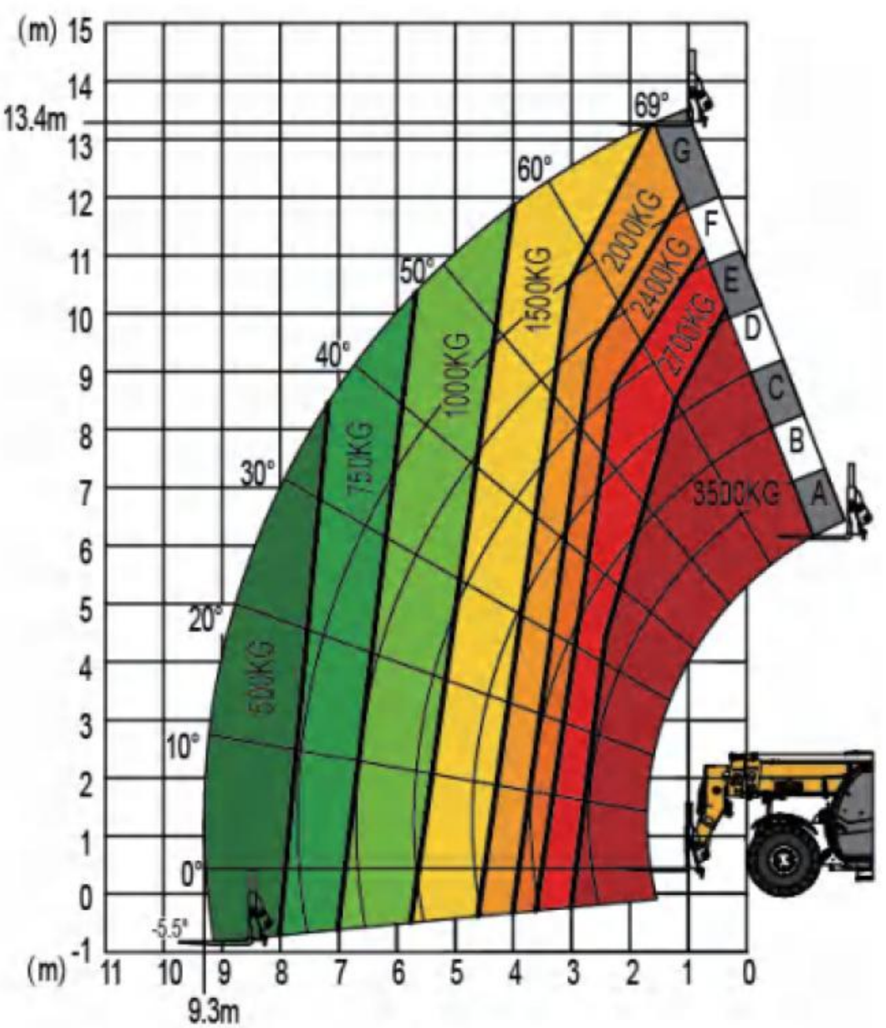
Range of motion GTH-XT3514K with stabilizers up
